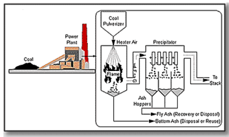
Figure 1. Production of fly ash in a dry-bottom utility boiler with electrostatic precipitator.
